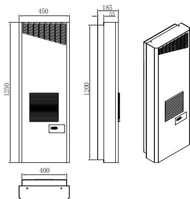
FCC1100P/1500P dimension drawing & cutout drawing :
