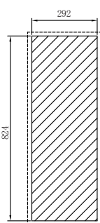
FCC680Q/825Qcutout drawing:
