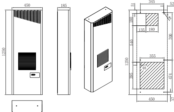
FCC1100P/1500P dimension drawing & cutout drawing :
