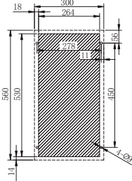
FCC225/320安装开孔图:
