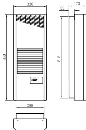
FCC680P/825Pdimension drawing & cutout drawing :
