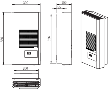
FCC225P/320P外形图和安装开孔图 :
