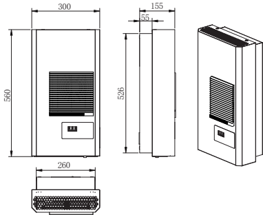
FCC225P/320Pdimension drawing & cutout drawing :
