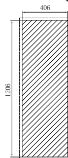
FCC1100Q/1500Q cutout drawing:
