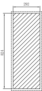
FCC680Q/825Q安装开孔图:
