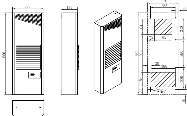
FCC680P/825Pdimension drawing & cutout drawing :
