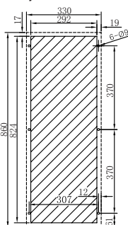
FCC680/825cutout drawing:
