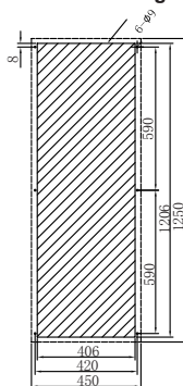
FCC1100/1500 cutout drawing:
