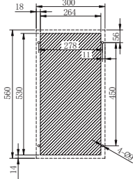
FCC225/320cutout drawing:
