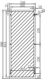
FCC680/825安装开孔图:
