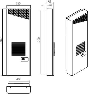
FCC1100P/1500P外形图和安装开孔图：
