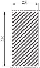
FCC225Q/320Q安装开孔图:
