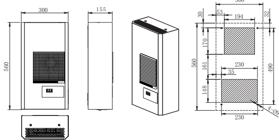
FCC225P/320Pdimension drawing & cutout drawing :
