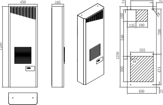
FCC1100P/1500P外形图和安装开孔图：
