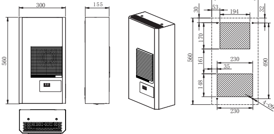
FCC225P/320P外形图和安装开孔图 :
